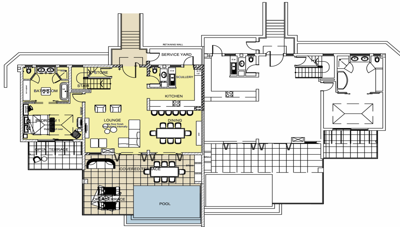
MOUNTAIN VILLA - 3 BEDROOM (Medium Slope) GROUND FLOOR PLAN
