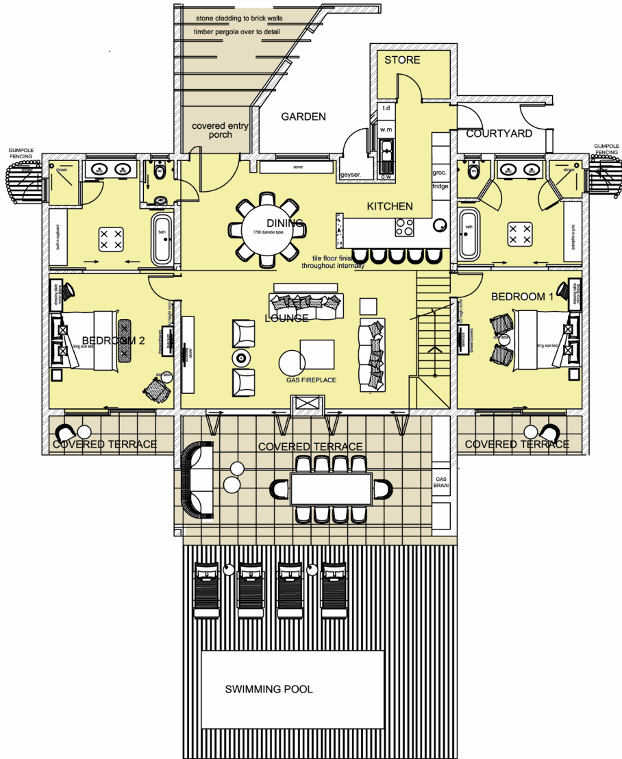
VALLEY VILLA - 4 BEDROOM (Alt 2) GROUND FLOOR PLAN
